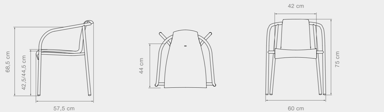
23801 NAMI Dining chair, armrest
