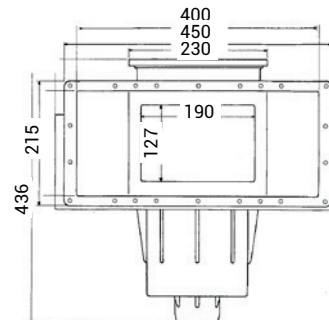
Skimmer dimension - wide track 3119
