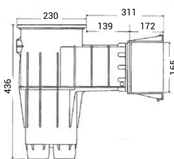
Skimmer dimension - wide track 3119
